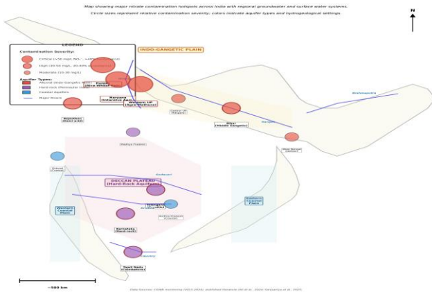
Figure 3: Spatial-Temporal Distribution and Hydrogeological Controls
