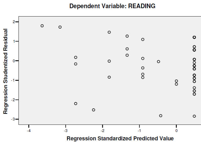
Figure 3 : Scatter plot
